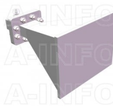
LB-159-15-C-NFSPO Standard Gain Horn Antenna 4.9-7.05GHz 15dB Gain N Type Female
