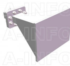
LB-159-15-C-3.5FSPO Standard Gain Horn Antenna 4.9-7.05GHz 15dB Gain 3.5mm Female
