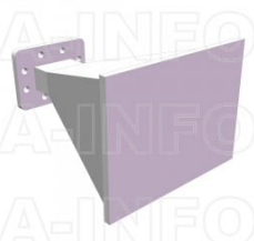
LB-159-15-ASPO Standard Gain Horn Antenna 4.9-7.05GHz 15dB Gain Rectangular Waveguide Interface
